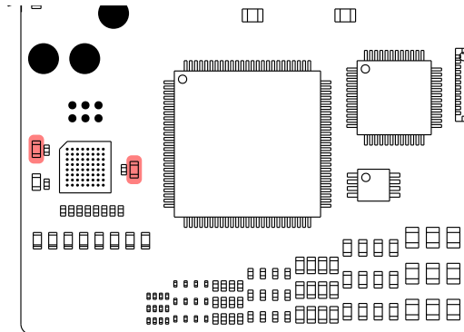
C7 C6 2x 2μ2 0603-L Farnell 2496923
