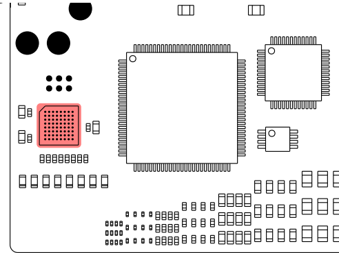
IC3 1x STM32F091RxHx UFBGA-64 Farnell 2503242
